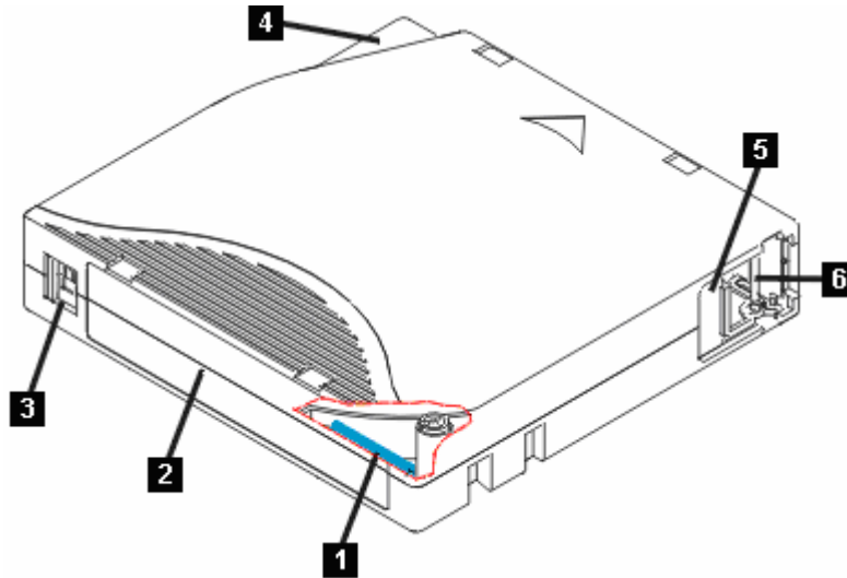
Figure 14 LTO Ultrium Data Cartridge
