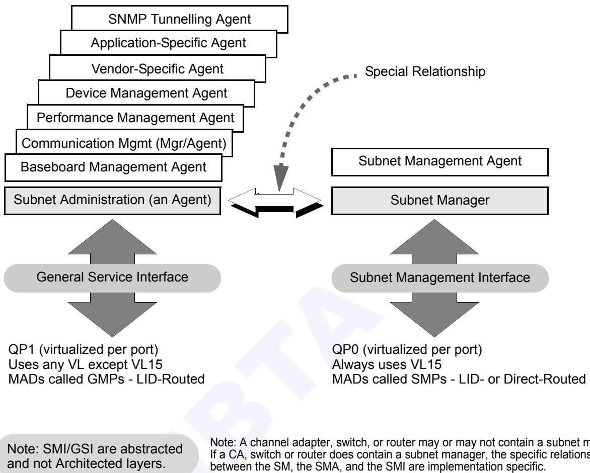
Figure 153 MAD Interface
