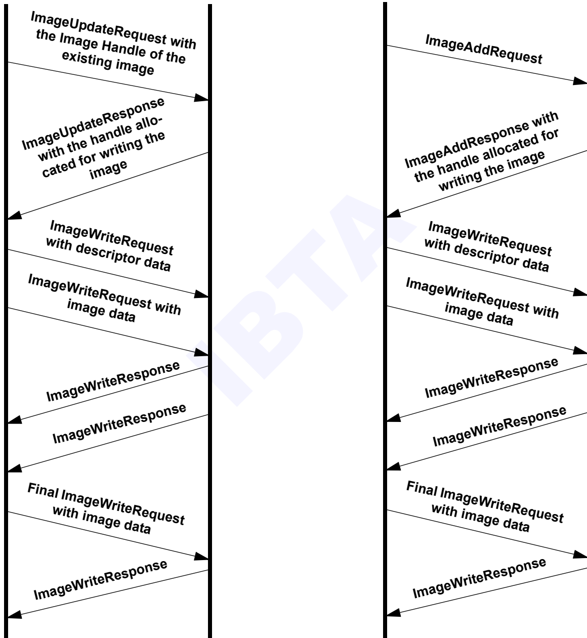
Figure 287 Ladder Diagram of Image Write operation
