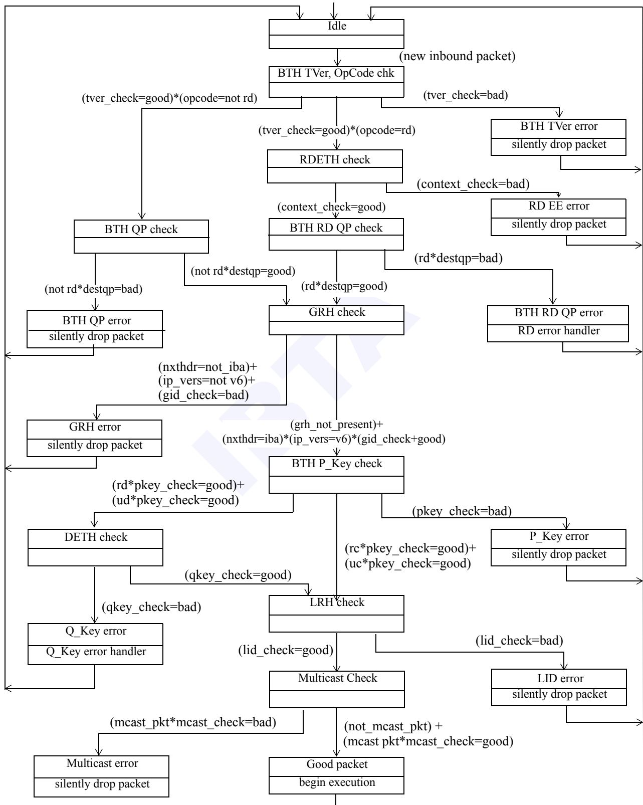
Figure 81 Packet Header Validation Process
