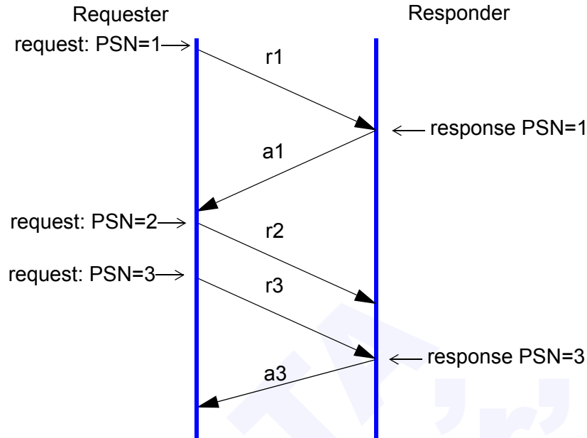
Figure 90 Example: PSNs for Response Messages
