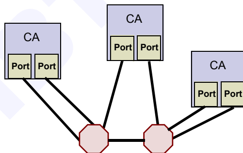
Figure 216 Multiported CAs Connected to Single Subnet
