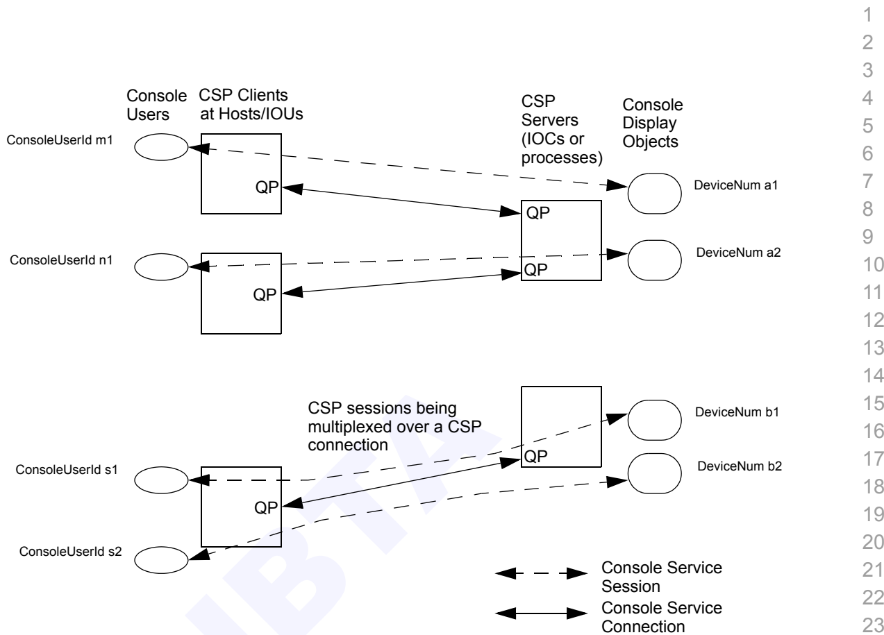
Figure 231 Schematic of IBA Console Abstraction
