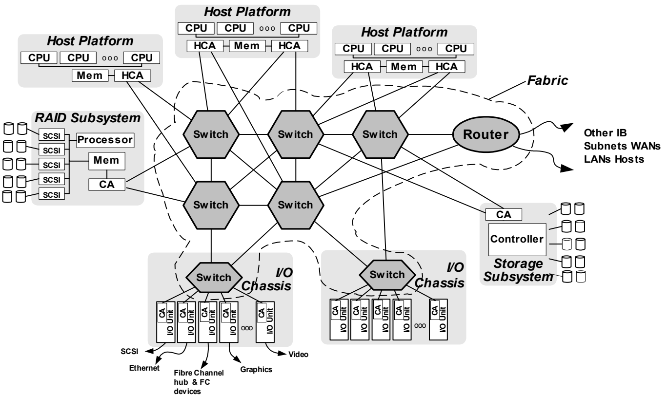
Figure 228 Multiple Systems
