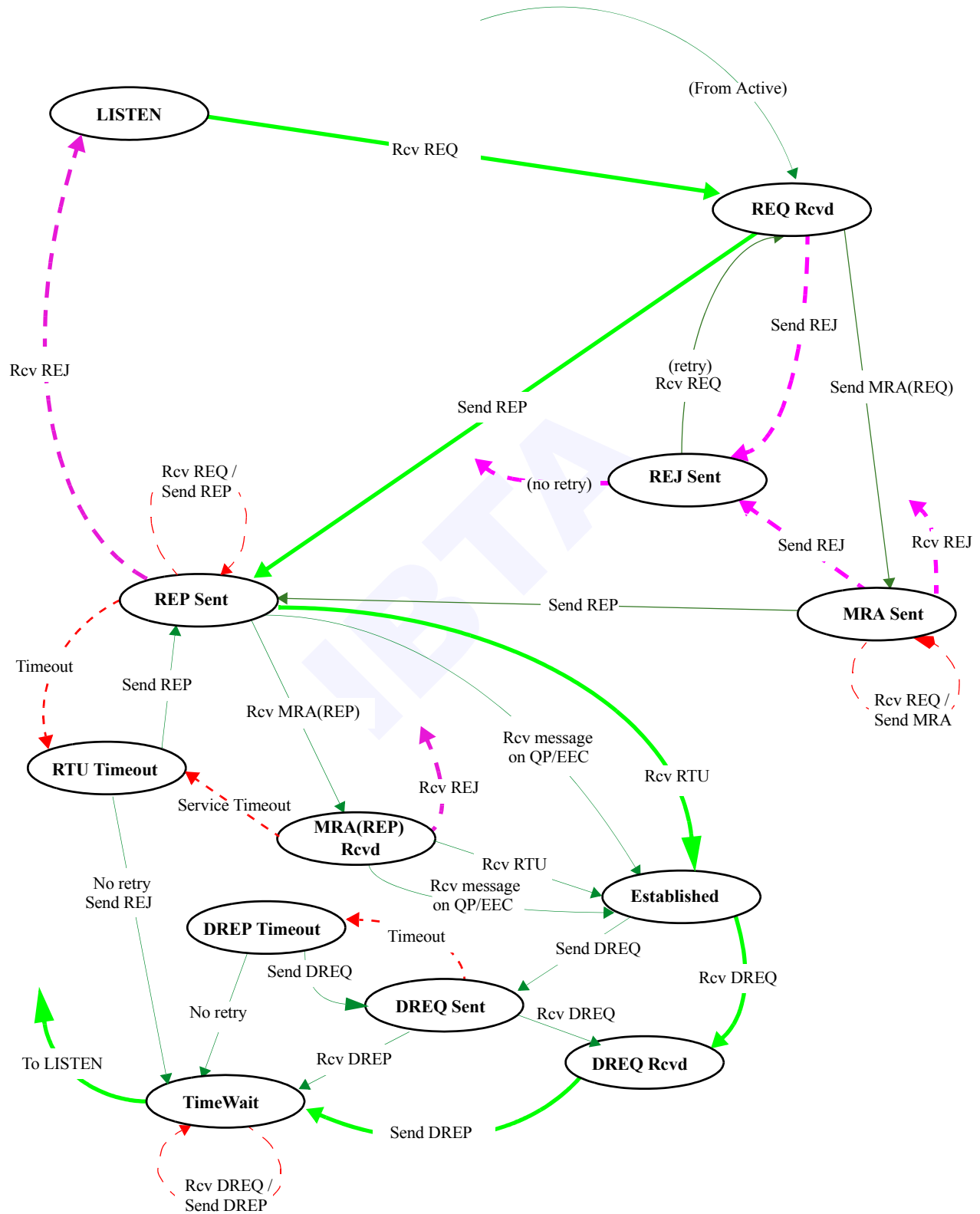
Figure 132 Communication Establishment(Passive Side)
