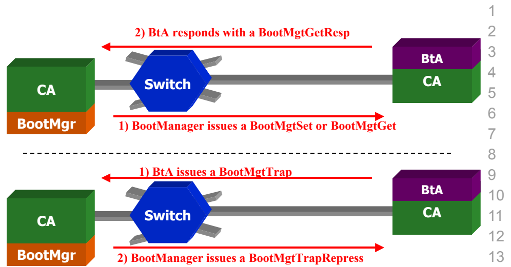
Figure 273 BootManager/BtA Relationship
