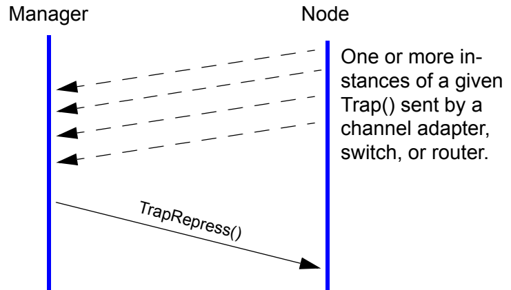
Figure 149 TrapRepress()
