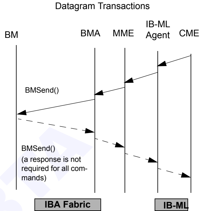
Figure 202 IB-ML Initiated Command
