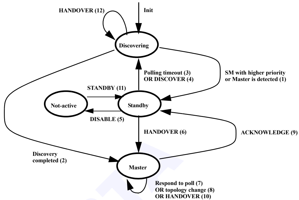
Figure 194 SMInfo State Transitions
