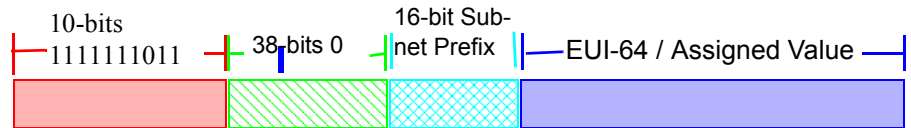
Figure 40 Site-Local Unicast GID Format
