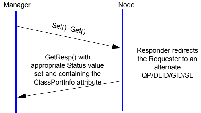
Figure 154 GSI Redirection
