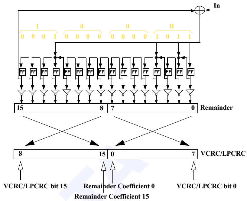
Figure 57 VCRC / LPCRC Generator
