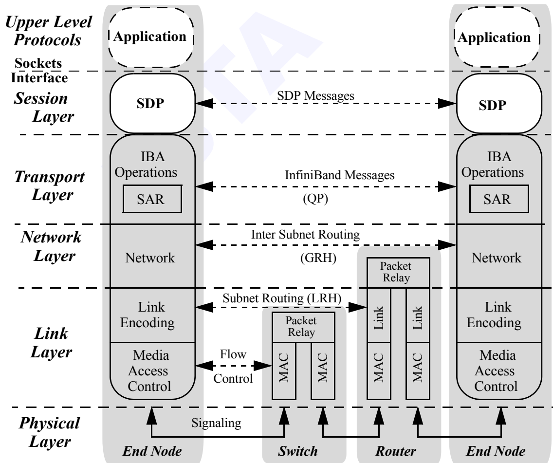
Figure 250 SDP Relation to IBA Architecture Layers
