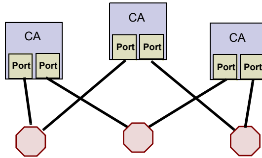
Figure 217 Multiported CAs Connected to Multiple Subnets
