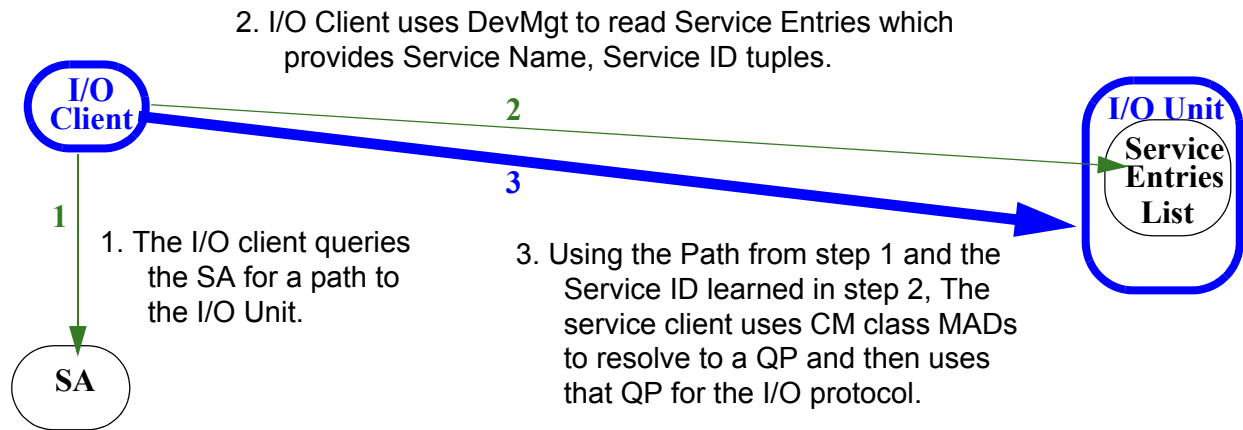
Figure 243 Typical Service Resolution for I/O Services
