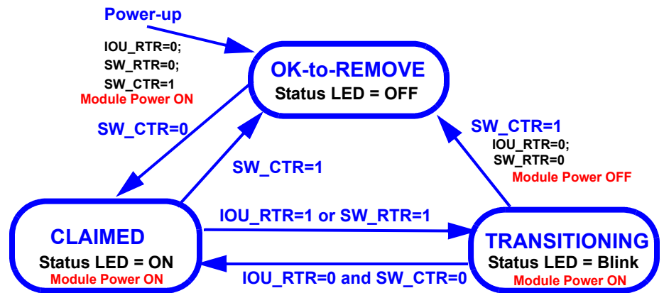
Figure 321 Graceful Removal State Diagram
