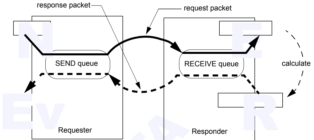
Figure 87 Request/Response PSNs
