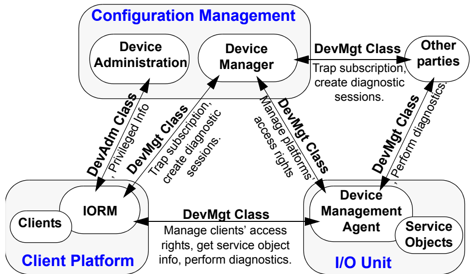
Figure 293 Configuration Management Usage Model
