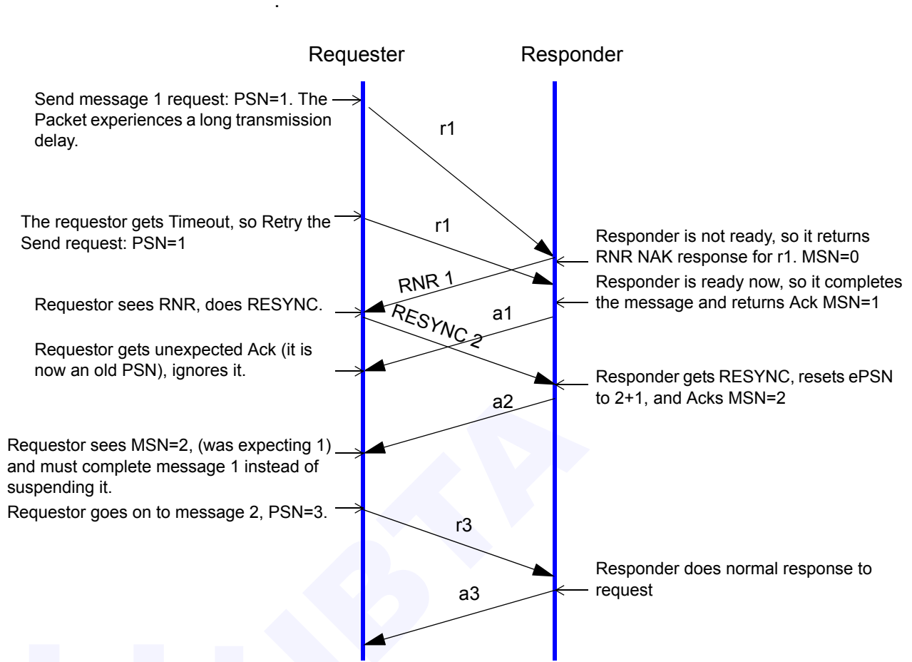
Figure 109 RESYNC detects unexpectedly complete message
