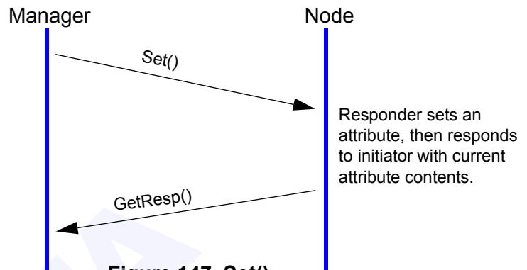
Figure 147 Set()
