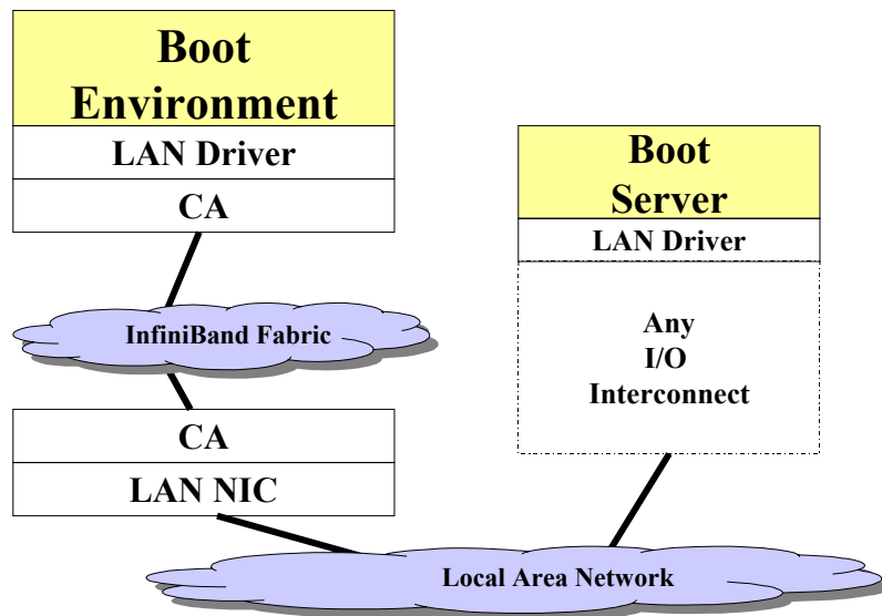
Figure 271 LAN Network Boot Model
