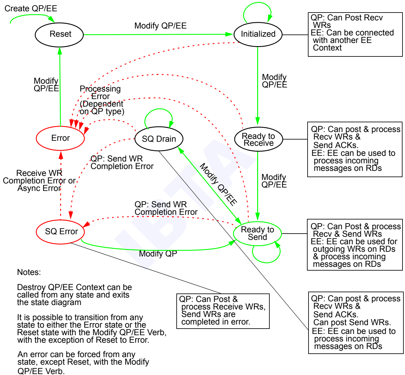
Figure 124 QP/EE Context State Diagram
