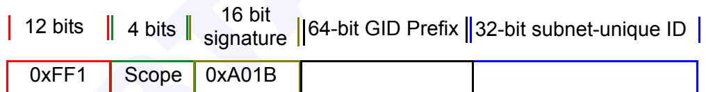
Figure 196 SA-Created Multicast GID Format
