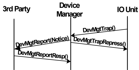
Figure 300 Trap Forwarding
