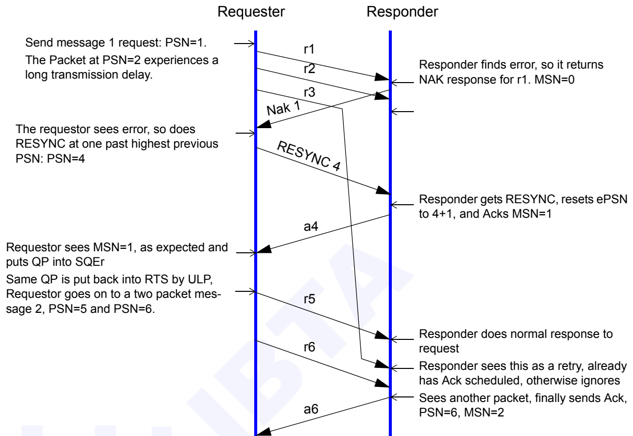
Figure 110 RESYNC prevents corruption by delayed packets
