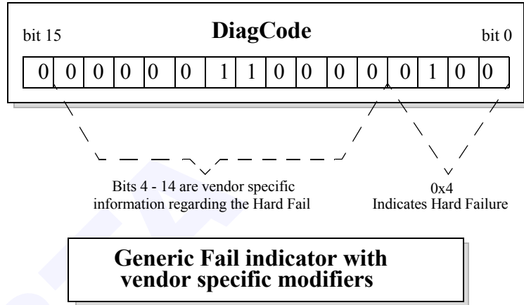
Figure 191 Example of DiagCode Bits
