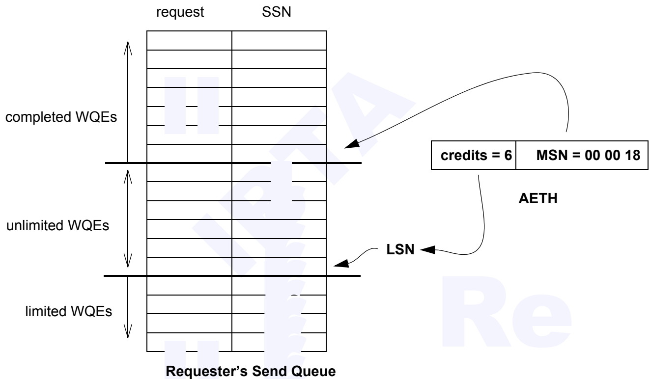
Figure 105 Relating AETH values to the Send Queue
