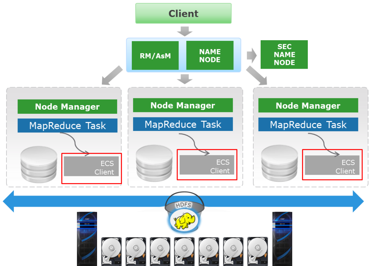
Figure 2. ECS HDFS Data Service Architecture
