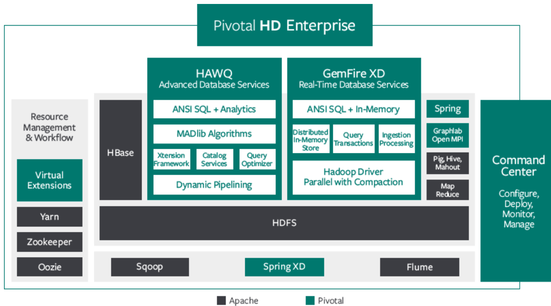
Figure 1. Apache Hadoop Components (Source: Pivotal, Inc.)
